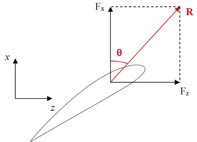
Fig. 5. Frame of reference for the calculation of the magnitude ( R ) and angle ( \theta ) of the hydrodynamic resultant.
