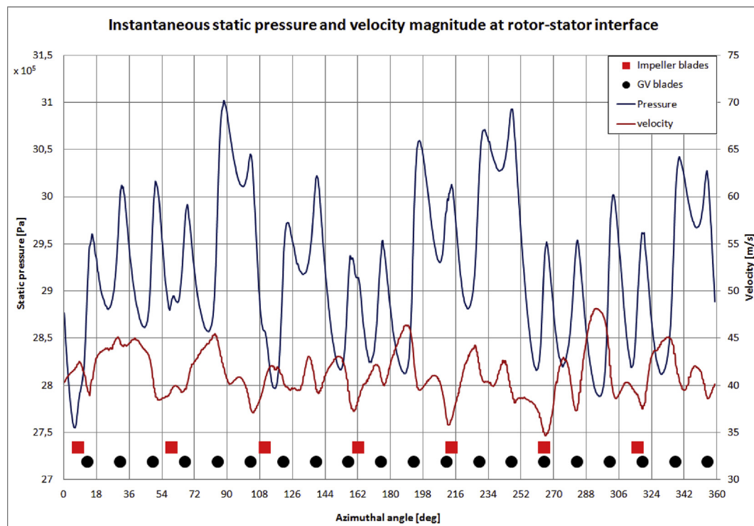
Fig. 10. Azimuthal static pressure and velocity magnitude distribution at a constant radius within the rotor-stator interface for GV opening angle 18^\circ . Red squares are the trailing edge impeller blade positions. Black dots are the trailing edge GV blade positions. Radius and instant of time equal to Fig. 9.
