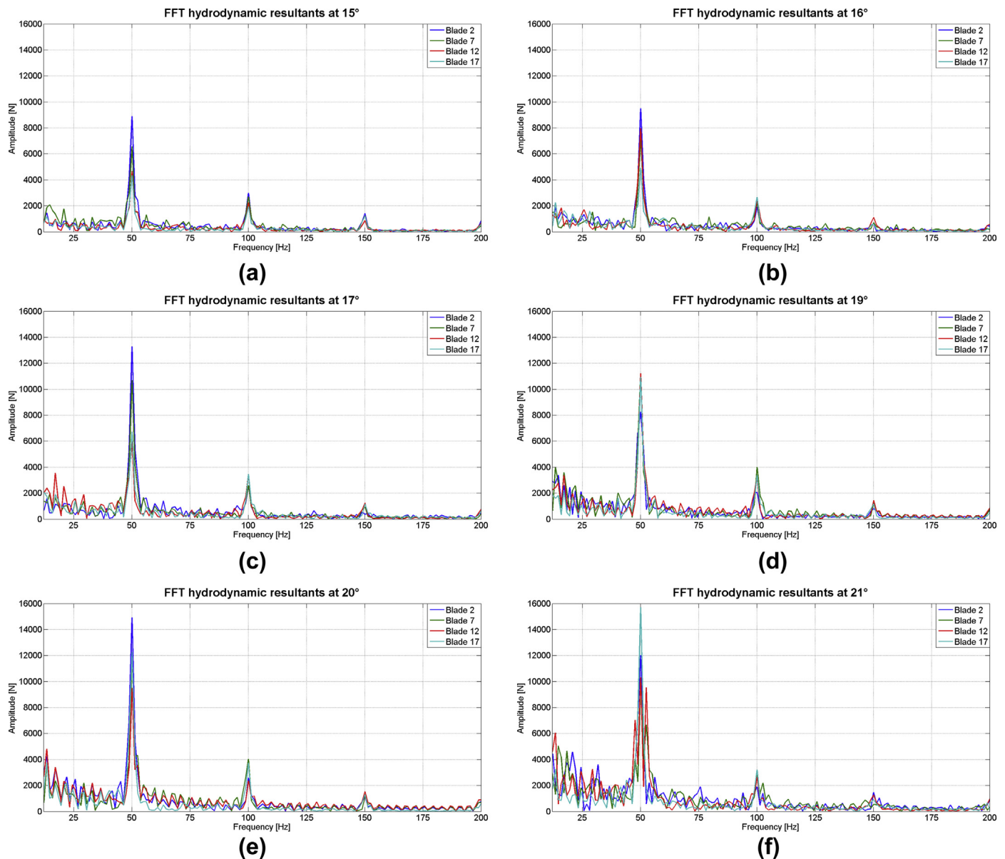
Fig. 18. Fast Fourier transform of the time-dependent hydrodynamic resultant magnitude for GV blade opening angles 15^\circ (a), 16^\circ (b), 17^\circ (c), 19^\circ (d), 20^\circ (e), 21^\circ (f) for blades 2, 7, 12 and 17 (see Fig. 11 for reference).
