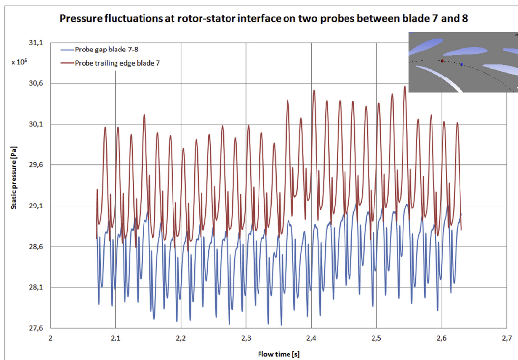
Fig. 12. Time-dependent pressure fluctuations sampled on two probes at a circumference within the rotor-stator interface at a mid-span for GV opening angle 18^\circ , for two consecutive azimuthal positions. Red line refers to a probe near the trailing edge of blade 7. Blue line refers to a probe placed on the gap between blade 7 and 8.
