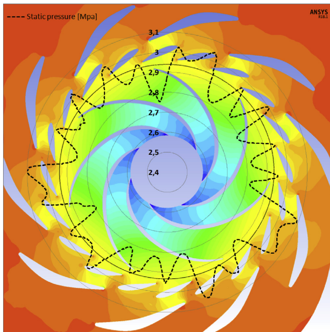
Fig. 9. Azimuthal static pressure distribution at a constant radius (black circle at a mid-span section) within the rotor-stator interface for GV opening angle 18^\circ superimposed on instantaneous static pressure contours at the same mid-span section.
