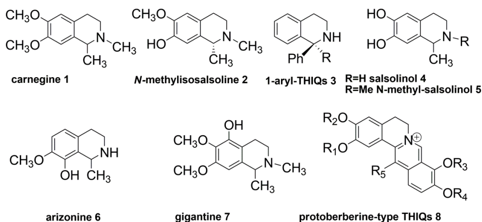
Figure 1. Structure of some natural and synthetic 1,2,3,4-tetrahydroisoquinoline (THIQ) alkaloids.
