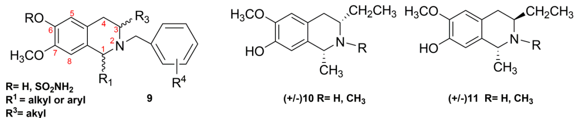
Figure 2. Structures of the known C3/C1-substituted THIQs ( 9 ) endowed with antiproliferative activities and the C3/C1-substituted ( 10–11 ) THIQs reported herein.
