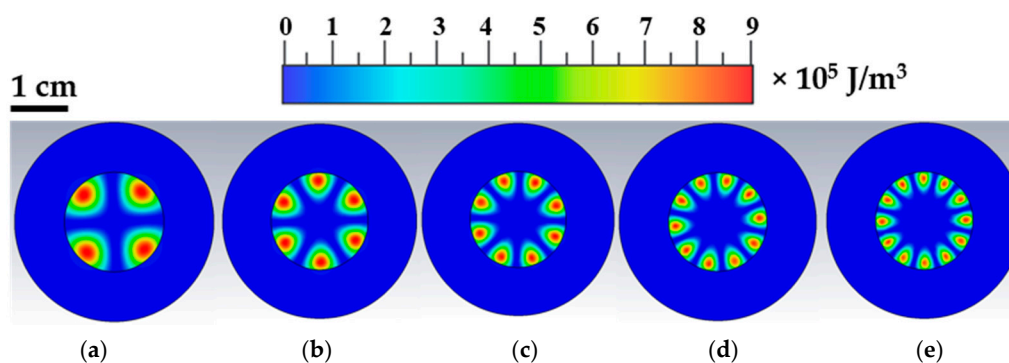
Figure 4. Computer electromagnetic simulations: electric energy densities at resonance. In the frequency range from 6 to 14 GHz, five WGM resonances have been found: (a) \text{WGM}_{n=2} ; (b) \text{WGM}_{n=3} ; (c) \text{WGM}_{n=4} ; (d) \text{WGM}_{n=5} and (e) \text{WGM}_{n=6} . The five panels report the expected electromagnetic field distribution at the WGM resonances.
