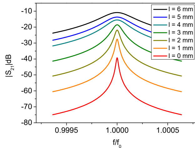
Figure 2. Magnitude of the resonator transmission coefficient ( S_{21} ) with different antennas length ( l ). Only the fitted Lorentzian function of the measured spectrum is reported here. The shorter are the antennas, the higher is the quality factor and the lower is the peak amplitude.
