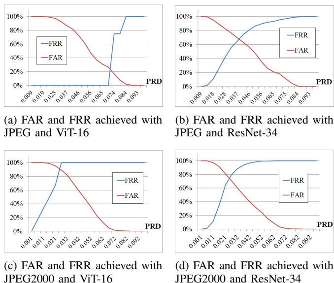
Fig. 6: FRR and FAR achieved with different models and compression algorithms.
