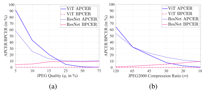
Fig. 3: PAD performance for varying compression levels. (a): JPEG; (b): JPEG2000.
