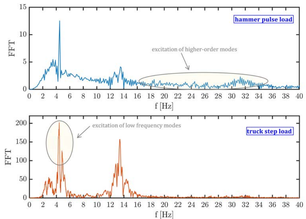
Figure 7. FFT of the S1 signal under hammer pulse load ( top ) and truck step load ( bottom ).
