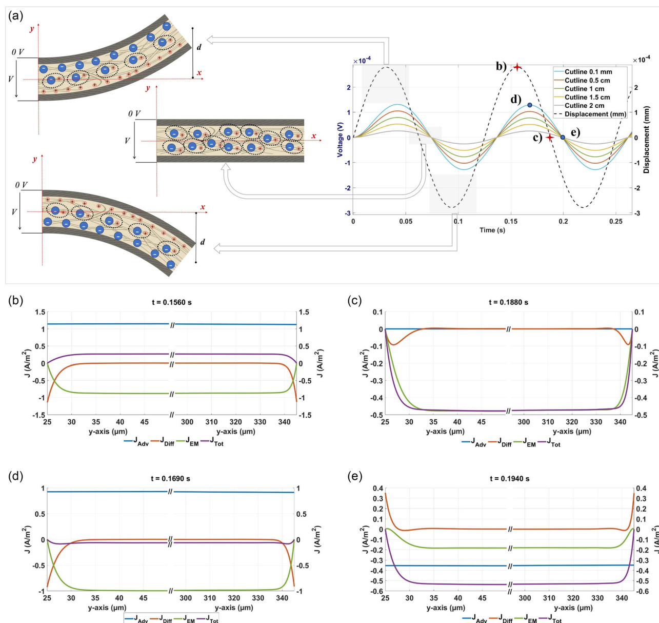
Figure 7. Simulation results for the BC–IL sensor under dynamic excitation. a) Simulated voltage responses at various positions along the beam length, CL_{0.1\text{ mm}} , CL_{0.5\text{ cm}} , CL_{1\text{ cm}} , and CL_{2\text{ cm}} , illustrating the spatial dependence of the electrical output. The panel also includes a schematic illustration of the dual-ion sensing mechanism, highlighting the redistribution of cations and anions at positive displacement, negative displacement, and close to zero displacement. b, c) Spatial profile on the y -axis CL_{0.1\text{ mm}} cutline of the total ionic current density and its components (diffusion, electromigration, and advection) at key points of the displacement cycle: (b) maximum displacement and (c) zero displacement during the falling edge. d, e) Spatial profile on the y -axis CL_{0.1\text{ mm}} cutline of the ionic current density at characteristic points of the sensor voltage waveform: d) voltage peak and e) zero voltage during the falling edge.
