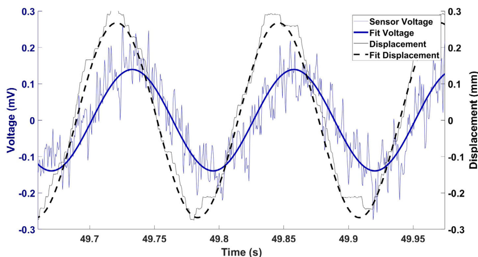
Figure 4. Experimental response of the BC sensor infused with EMIM-BF 4 to sinusoidal input displacements with amplitude d_{\text{MAX}} = 0.27 mm and frequency f_d = 8 Hz. The recorded signals were fitted using single-frequency sinusoids to filter noise and accurately extract amplitude and phase shift parameters.
