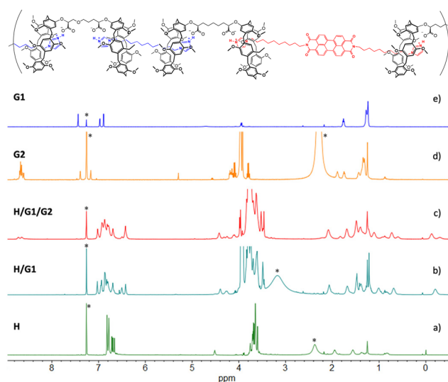
Fig. 5 ^1\text{H} NMR spectra (500 MHz, 25 °C, \text{CDCl}_3/\text{TFE} , 97 : 3, v/v) of: (a) [\text{H}] = 10 mM; (b) [\text{H}] = [\text{G1}] = 10 mM; (c) [\text{H}] = 10 mM, [\text{G1}] = 9 mM, [\text{G2}] = 1 mM; (d) [\text{G2}] = 0.6 mM. *Asterisks refer to residual solvent peaks.
