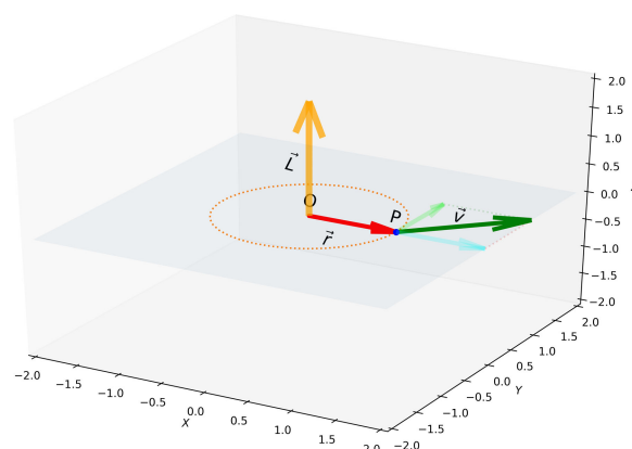
FIGURE 1. The angular momentum, computed as vector product using NumPy, and plotted with Matplotlib.
