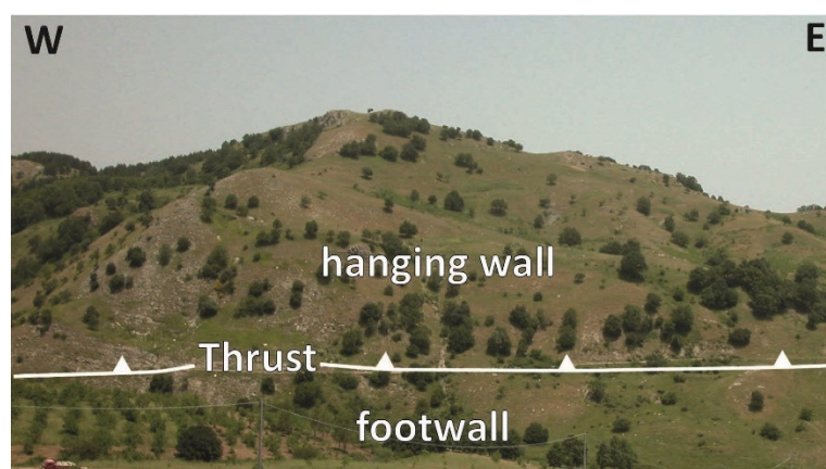
Figure 18. GS12—Peloritani Thrust Front in the central sector of the Taormina Line. In this panoramic view of Pizzo Leo, it is possible to observe the thrust of the Longi-Taormina Unit (hanging wall) on the Units of the Maghrebian Flysch Basin (footwall).
