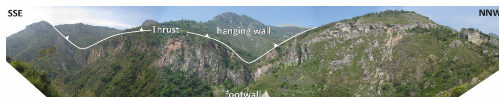
Figure 13. GS08—Thrust at the Monte Veneretta–Monte Pernice ridge. Aesthetic panoramic view of the frontal ramp and the landscape. The thrust cuts the Paleozoic to Meso-Cenozoic succession of the Longi-Taormina Unit.
