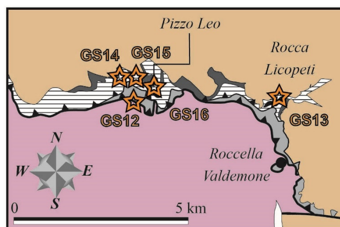
Figure 17. Geological sketch map of the Roccella Valdemone area with the inventoried GS12 to GS16 possible geoheritage sites. For localization of the geological map and the legend, see Figures 3 and 12, respectively.
