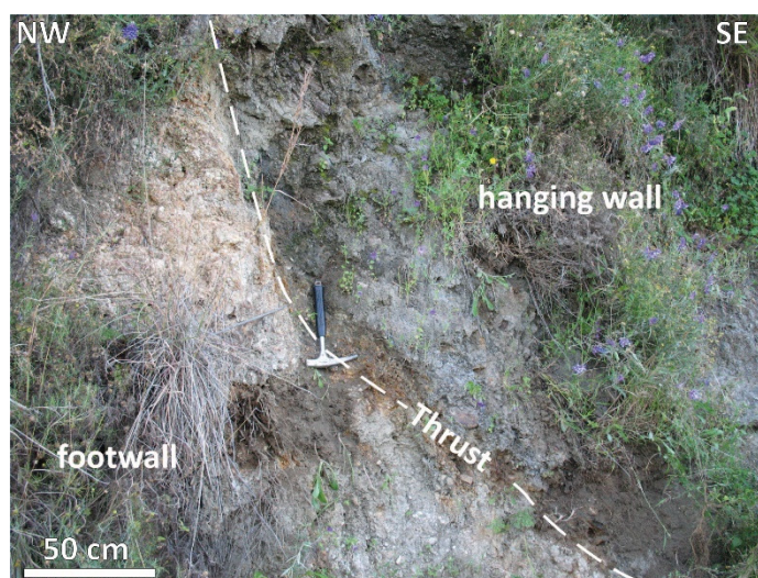
Figure 9. GS05—Modderino klippe. In this outcrop, it is possible to observe a detail of the thrust.
