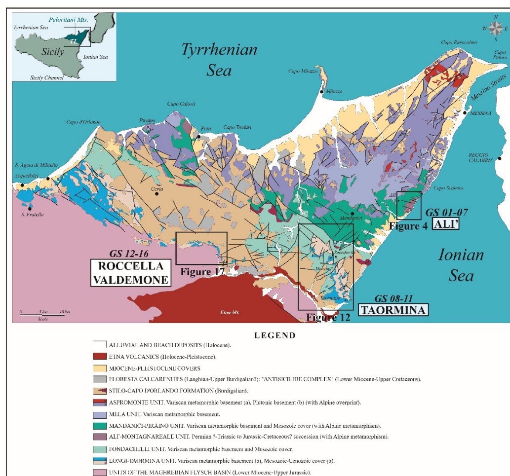
Figure 3. Geological sketch map of the Peloritani Mountains showing the three studied areas (Ali, Taormina, Roccella Valdemone) and the related sixteen sites showing geodiversity elements (GS01-16). In the insert, the geographical position of the Peloritani Mountains is shown with the localization of the Taormina Line (TL).
