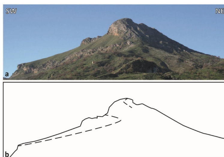
Figure 15. GS10—Fold at Monte Galfa. Aesthetic panoramic view of the fold and landscape. The fold is observable on the photograph (a) and drawing (b).
