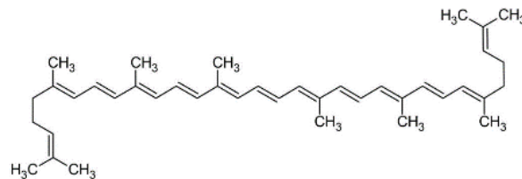
Figure 6. Structural formula of Lycopene.
