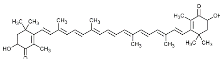
Figure 3. Structural formula of astaxanthin.
