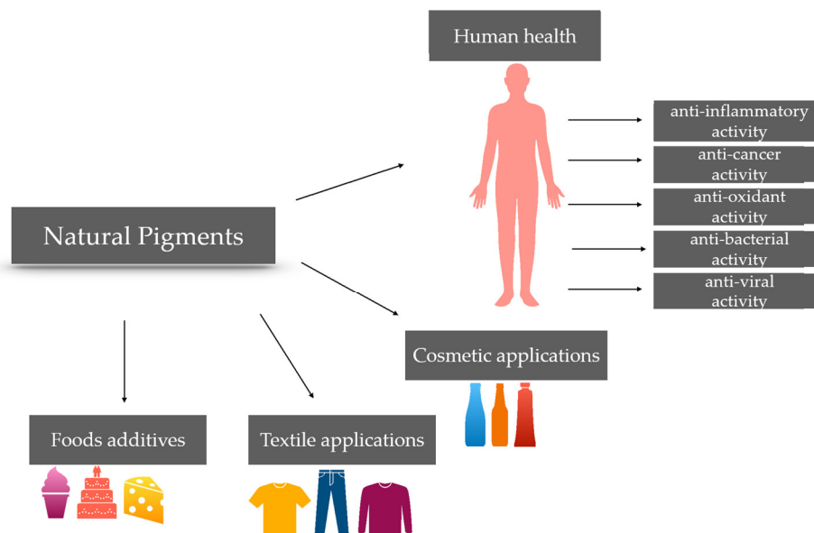
Figure 11. Summary diagram of the applications of natural pigments.
