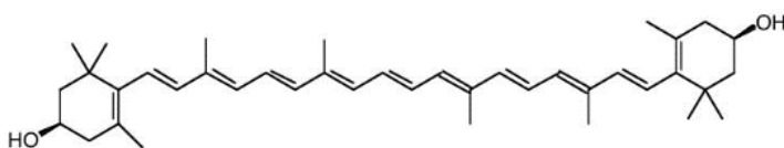
Figure 4. Structural formula of zeaxanthin.
