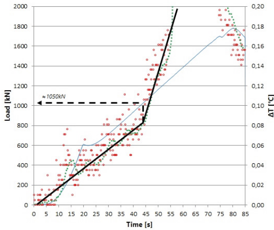
Fig. 4. \Delta T vs time curve (red points) and stress vs time curve (blue line) for spot number 5.
