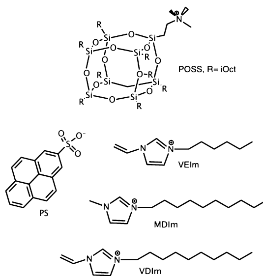
Scheme 1. Schematic Representation and Abbreviations of PS Adducts
