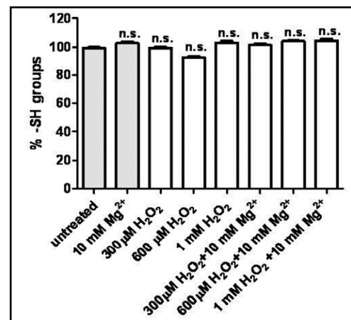
Fig. 4. Percentage of membrane -SH groups measured in untreated erythrocytes, or Mg^{2+} -treated (control) or treated with either 300 \mu M or 600 \mu M or 1 mM H_2O_2 with or without 10 mM Mg^{2+} (10 mM Mg^{2+} + 300 \mu M H_2O_2 or 10 mM Mg^{2+} + 600 \mu M H_2O_2 or 10 mM Mg^{2+} + 1 mM H_2O_2 ). Bars represent the mean \pm SD from at least 5 experiments, where 10 mM Mg^{2+} n.s. versus untreated erythrocytes; n.s. versus control.
