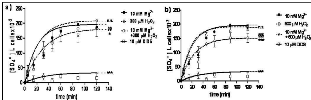
Fig. 2. Time course of SO_4^{=} uptake in human erythrocytes measured in control conditions (10 mM Mg^{2+} ) or in erythrocytes treated with 300 \mu M H_2O_2 or 10 mM Mg^{2+} + 300 \mu M H_2O_2 (A); or with 600 \mu M H_2O_2 , or 10 mM Mg^{2+} + 600 \mu M H_2O_2 (B) or 10 \mu M DIDS (A,B). Points represent the mean \pm SD from at least 5 separate experiments (see Table 1), where n.s. is not significant, * p <0.05 and *** p <0.001 versus control; ^{ss} p <0.01 versus 300 \mu M H_2O_2 , ^{sss} p <0.001 versus 600 \mu M H_2O_2 .
