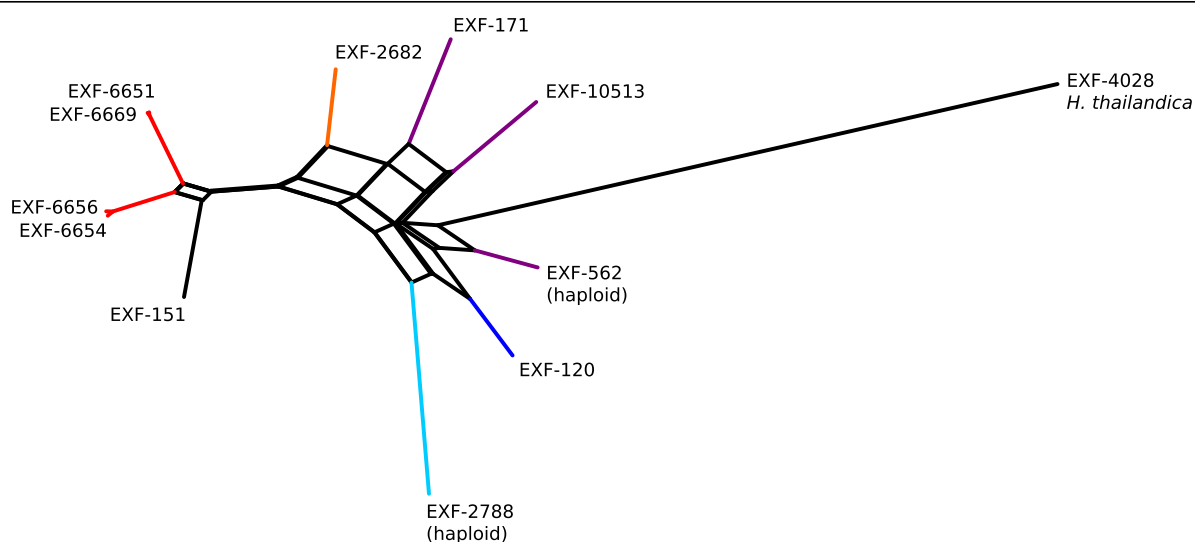
Fig. 5 Phylogenetic network of the Hortaera werneckii strains with sequenced genomes. The network was reconstructed with the Neighbour-Net algorithm based on the dissimilarity distance matrix calculated from the single nucleotide polymorphism data
