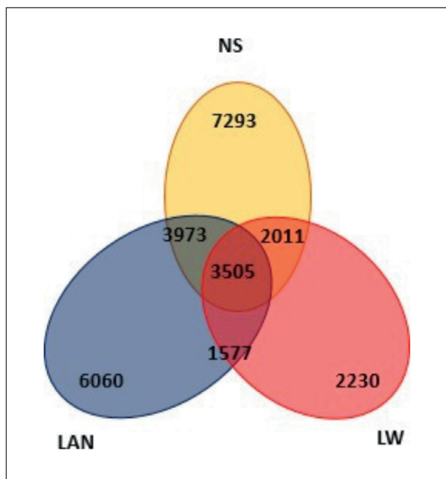
Figure 1 - Venn-Diagram showing shared (internal) and unshared (external) variant (SNPs and short INDEL) detected in this analysis.
