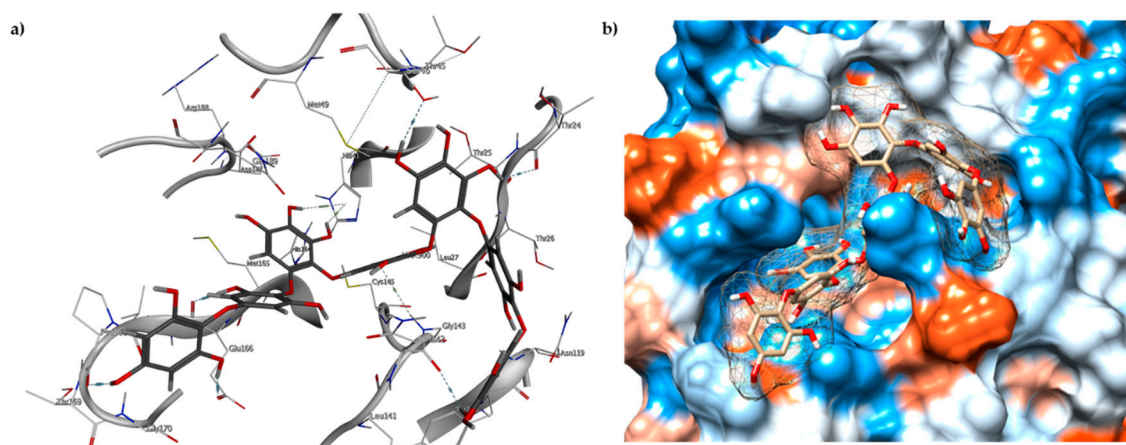
Figure 4. (a) Docked pose of 1 (grey, stick model) is shown with the binding pocket residues and interacting residues with M Pr (PDB ID: 6LU7); (b) View of 1 inside binding pocket in hydrophobic surface representation.
