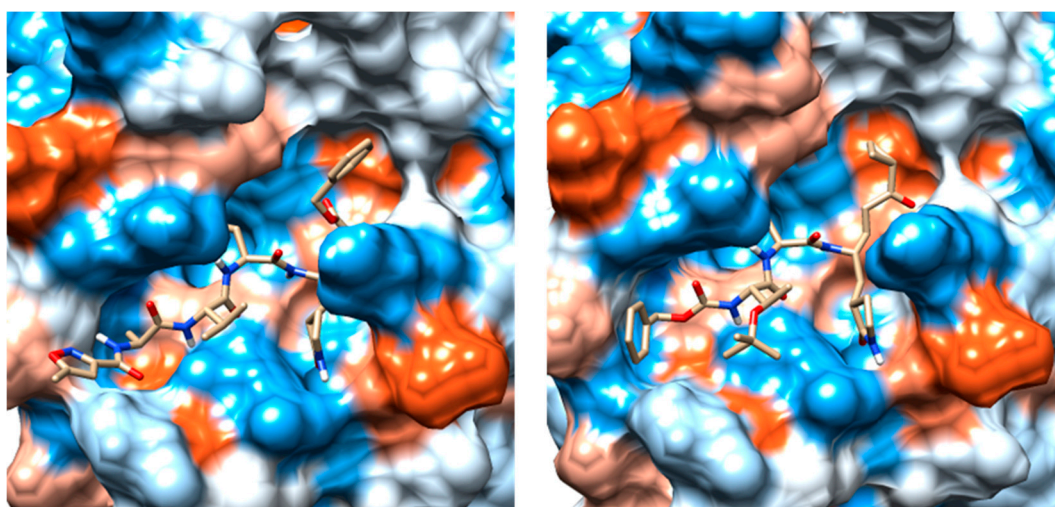
Figure 1. (a) Comparison between the binding pockets of the crystalline structure of the N3 inhibitor linked to the severe acute respiratory syndrome coronavirus 2 (SARS-CoV-2) main protease (M Pr ) (PDB ID: 6LU7); (b) the crystal structure of TG-0205486 inhibitor bound to the severe acute respiratory syndrome coronavirus (SARS-CoV-1) M Pr (PDB ID: 2ZU5).
