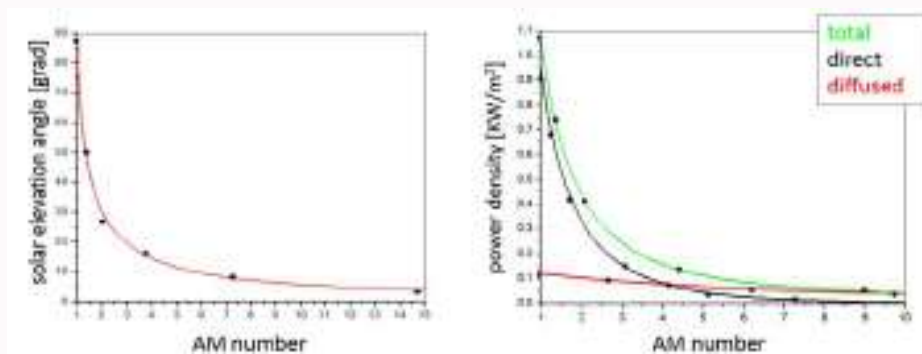
Figure 2: Air Mass number as a function of the solar elevation angle (on the left) and direct, diffused and total power density, according to AM number (on the right).
