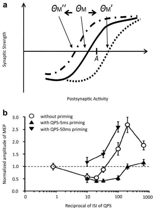
Figure 3. Figure shows the basic concept of metaplasticity following the BCM theory. The modification threshold ( \theta_M ), the crossover point from LTD to LTP, is not fixed but varies as a function of post-synaptic activity. Using an LTP-like prime will shift the modification threshold ( \theta_M' ) to the right along the x-axis, while using an LTD-like prime will shift the modification threshold ( \theta_M'' ) to the left on the x-axis. On the color bar, red codes an LTD response while blue codes an LTP response. (For interpretation of the references to colour in this figure legend, the reader is referred to the web version of this article.)
