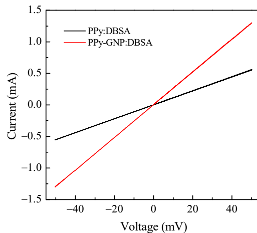
Figure 6. Current–voltage plots of PPy:DBSA and PPy-GNP:DBSA films.
