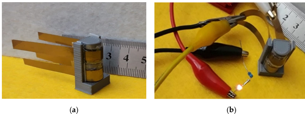
Figure 16. (a) Photograph of the sample holder used for bending tests. Two devices, each with an active area of about 1 cm 2 , were inserted into the stage, curvature radius of which was 5 mm; (b) picture taken 5 seconds after disconnecting the voltage supply used to charge the two capacitors (in series) inserted into the bending stage to 4 V: the LED remained lit by the charge stored in the devices for several seconds.
