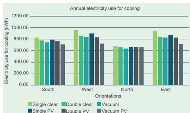
Fig. 8 | Annual cooling electricity consumption with different types of glazing in Hong Kong (source: YANG Hongxing).
