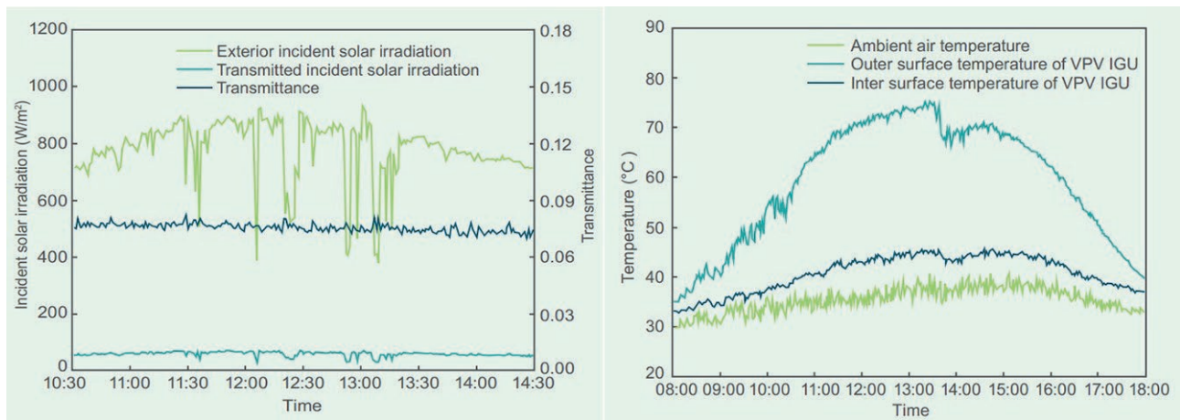
Fig. 7 | Transmission diagrams of incident solar radiation (source: YANG Hongxing).
